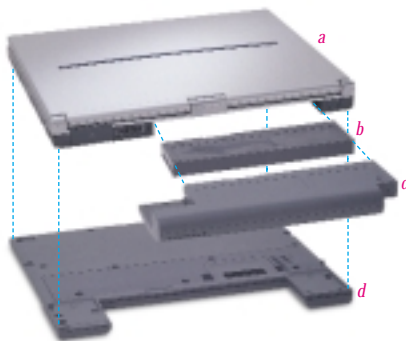
a: Versa FXi/FX b: Standard Battery (included) c: Extended-Life Battery (optional) d: Maximum-Life Battery (optional)
