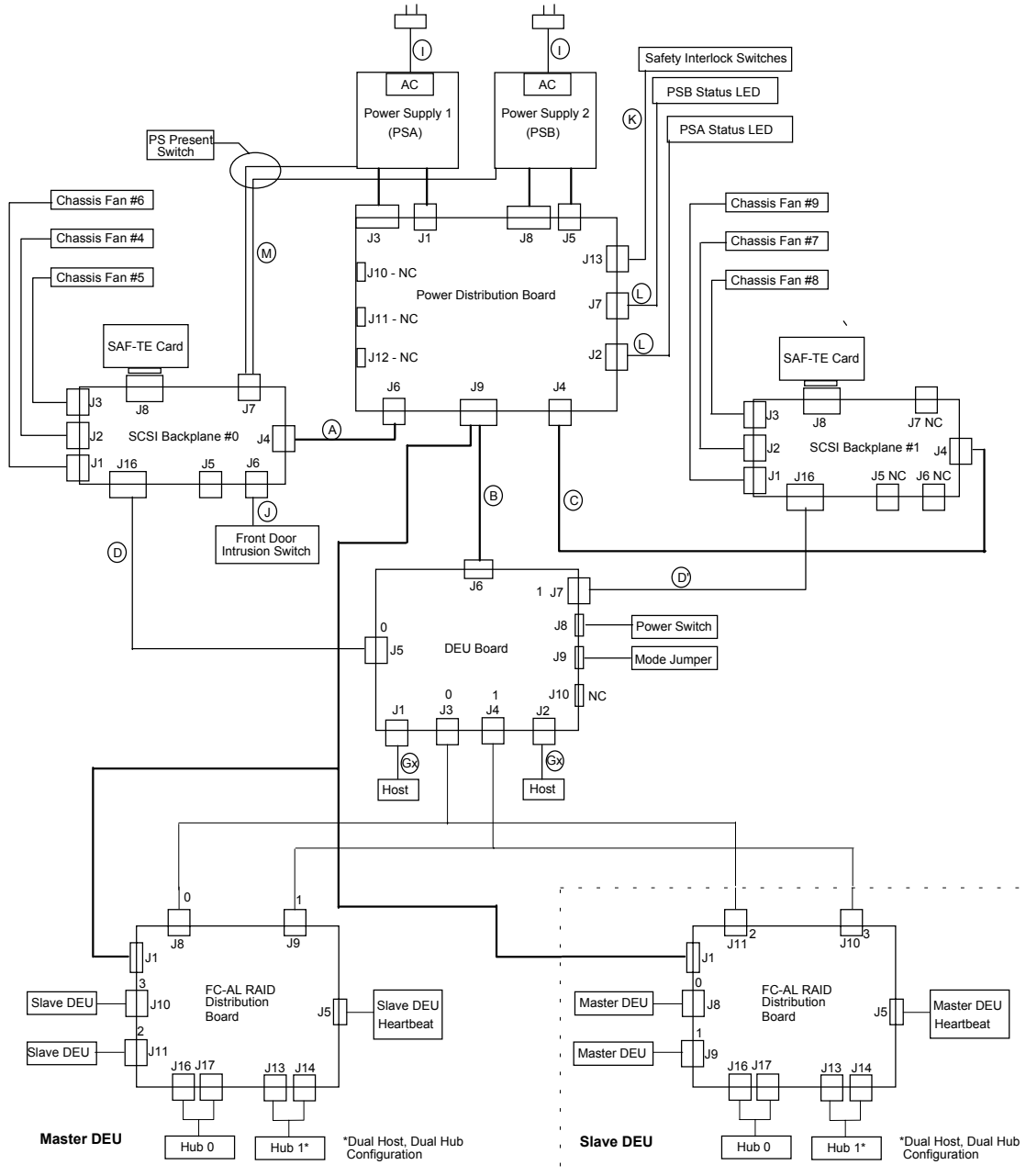
Figure 3-4. DEU Cabling (FC-AL)
